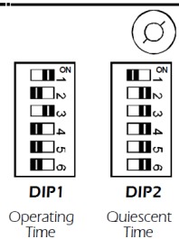
Selection of the operating timing at 10 min. And quiescent timing at 7 min., 45 sec.
